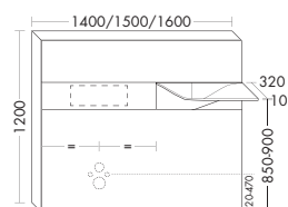
Version L - WT204 L
