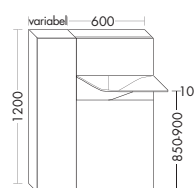
Version L - WT204 L
