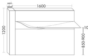
Version L - WT203 L
