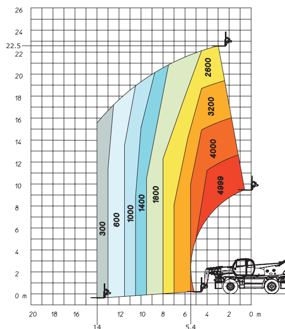
Rotation on extended stabilizers with winch 6000 kg
