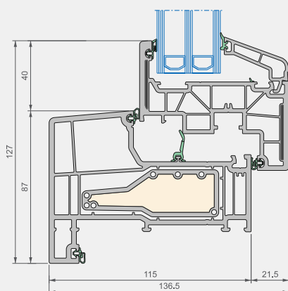
Elegant ThermoFibra Infinity 115 X verticaal
