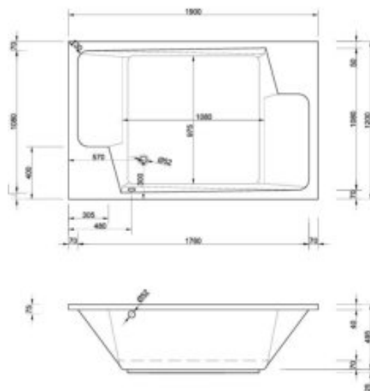
1900x1200x495mm, 485 Liter
