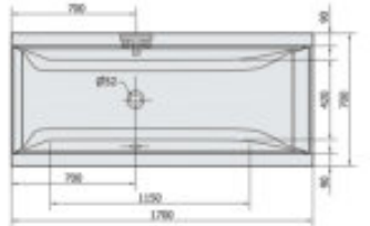
1700x700x480mm, 165 Liter
