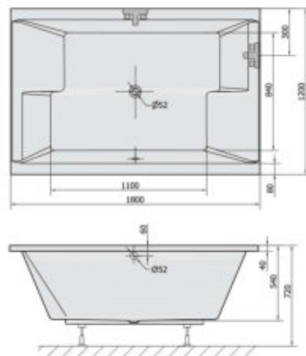
1800x1200x540mm, 500 Liter
