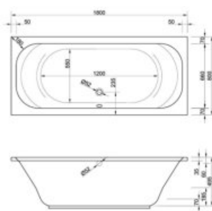
1800x800x495mm, 180 Liter
