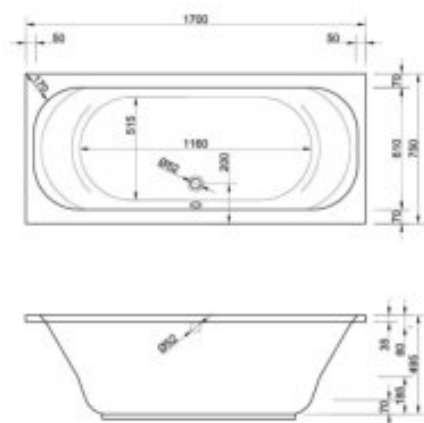
1700x750x495mm, 170 Liter
