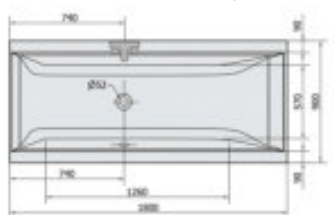
1800x900x480mm, 250 Liter
