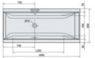
1800x800x480mm, 210 Liter
