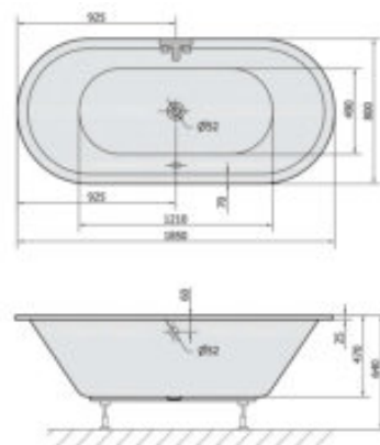
1850x800x470mm, 185 Liter
