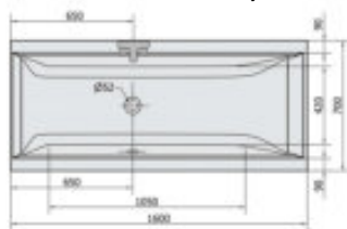
1600x700x480mm, 145 Liter
