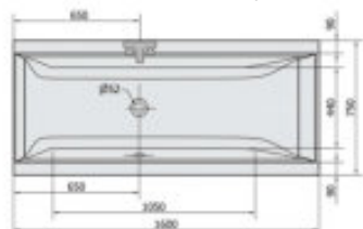
1600x750x480mm, 150 Liter
