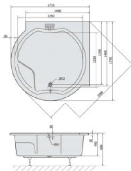
1720x1720x490mm, 495 Liter
