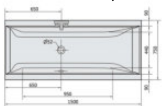
1500x750x480mm, 140 Liter
