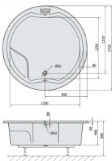
1720x1720x490mm, 495 Liter
