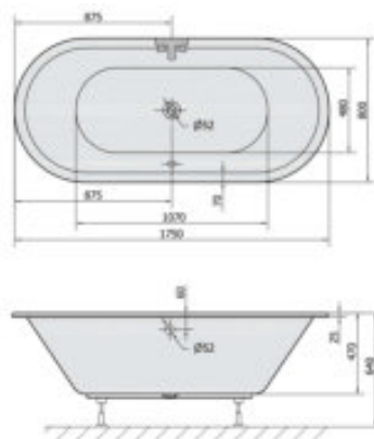
1750x800x470mm, 160 Liter
