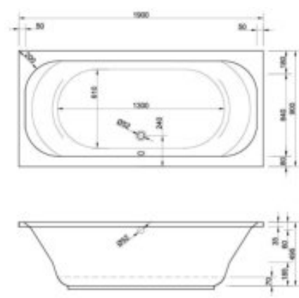
1900x900x495mm, 260 Liter
