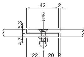
Stossdetail
