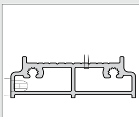
Seuil drainant PMR (17mm)
