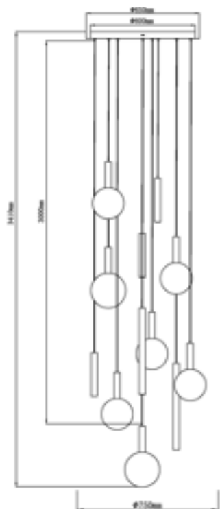
H 341 max. cm - W 75 cm - L 75 cm
