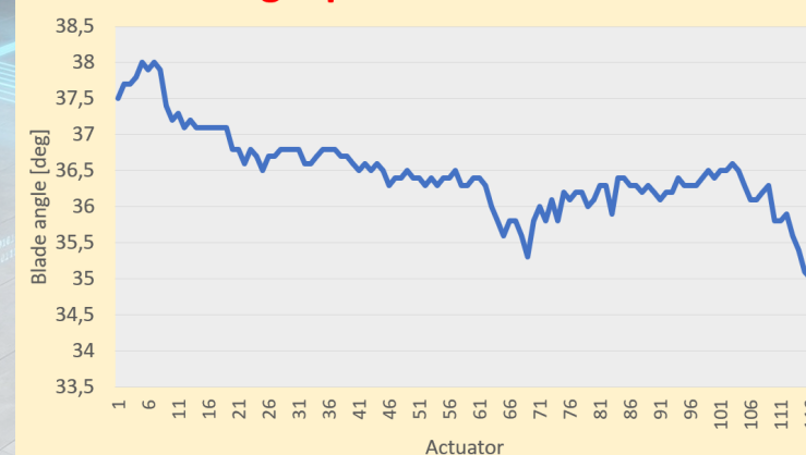
Blade angle profile with 1mm load
