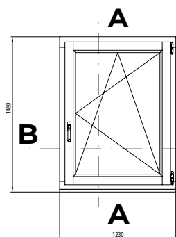
SECTION VERTICALE A-A
