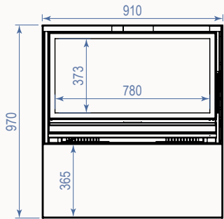
VENTILART PRO 90 DF/DK WOODBOX (Base Nordic Pro)
