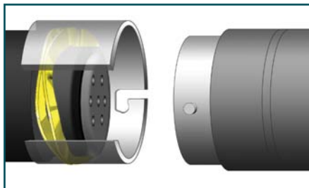
Bayonet Connector
