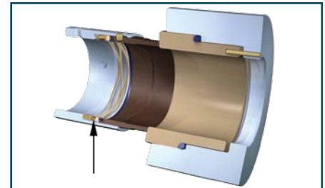
Mechanical Seal
