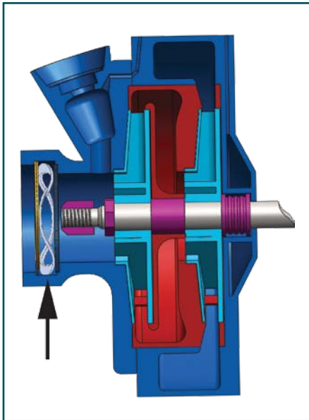
Centrifugal Pump
