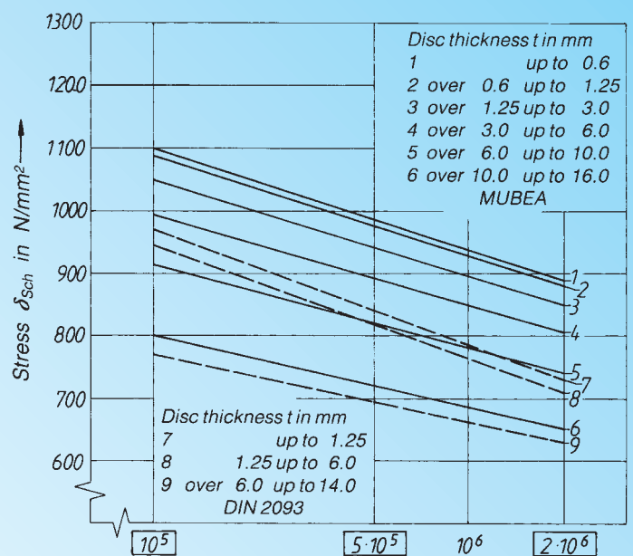
Woehler diagrams showing comparison between Mubea and DIN 2093
