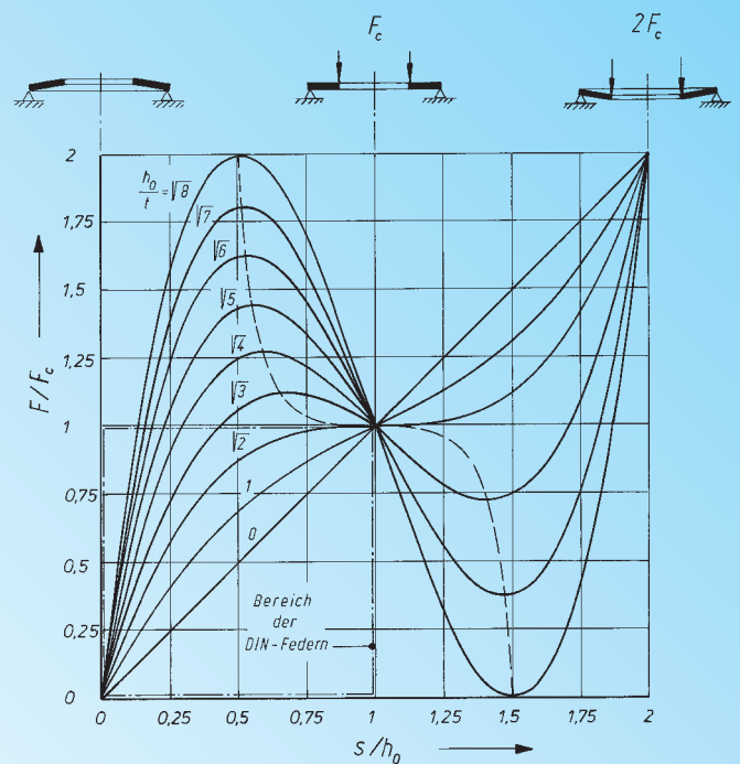
The relationship between disc spring height and material thickness ( h_0/t ) determines the characteristic load curve of the spring
