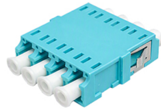
LC/LC-OM3-Quad-adapteri
