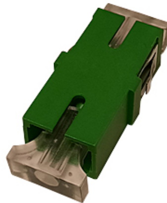
SCA/SCA-SM-simplex-adapteri (SC-APC)
