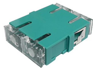
SC/SC-OM3-duplex-adapteri
