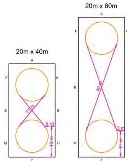
STEP 2: Diagonals
